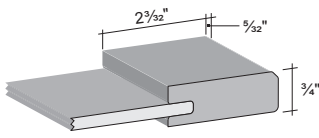
DRAWER FRONT PRESENTED DURHAM
