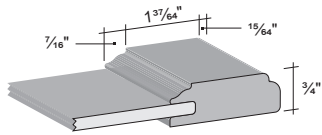
DRAWER FRONT PRESENTED BRIDGEWATER
