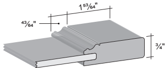
DRAWER FRONT PRESENTED LANCASTER 2 1/2"
