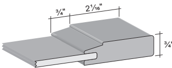
DRAWER FRONT PRESENTED BELLEVILLE
