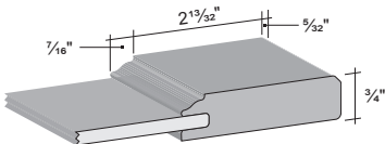
DRAWER FRONT PRESENTED LINCOLN 3" Rails width: 1 1/2"
