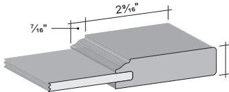
DRAWER FRONT PRESENTED KIRKLAND 3" Rails width: 1 1/2"
