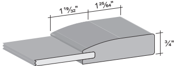
DRAWER FRONT PRESENTED AUGUSTA 3"
